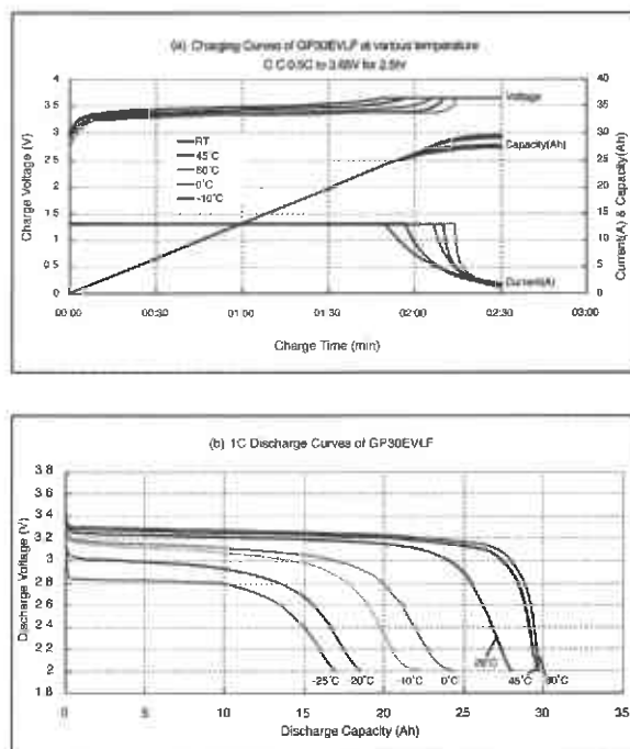
Figure 5 Performance Curves of LiFePO 4 Batteries
