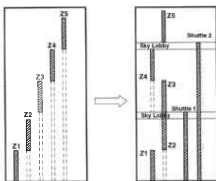
Figure 7 Skylobby Approach
