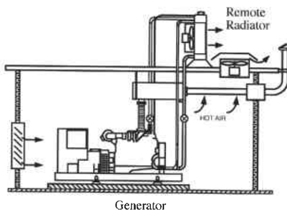
Figure 5 Remote Air-cooling
