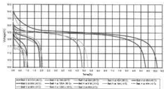
Figure 3 Storage Characteristics
