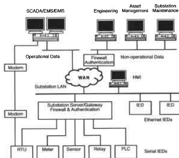
Figure 3 Securing the Integrated Substation Automation System
