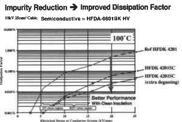
Figure 2 Dissipation Factor Improvement with Super Clean Compound
