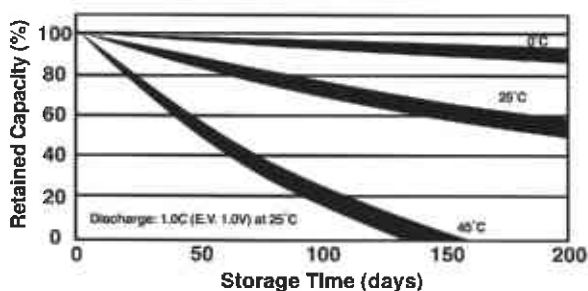
Figure 4 Charge Retention Test
